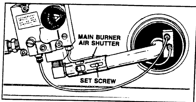
WATER HEATER BURNER ADJUSTMENT
