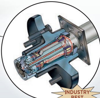
Ultralube axle bearing. Easier maintenance for improved safety
