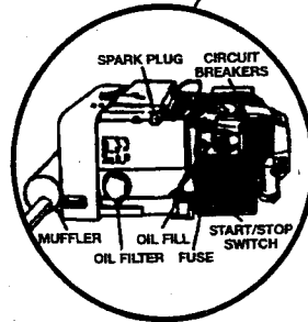
GENERATOR FIGURE 5
