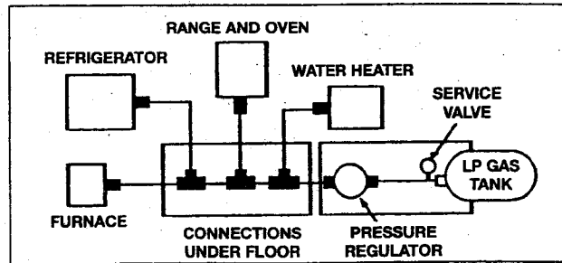
LP GAS SYSTEM (TYPICAL)
