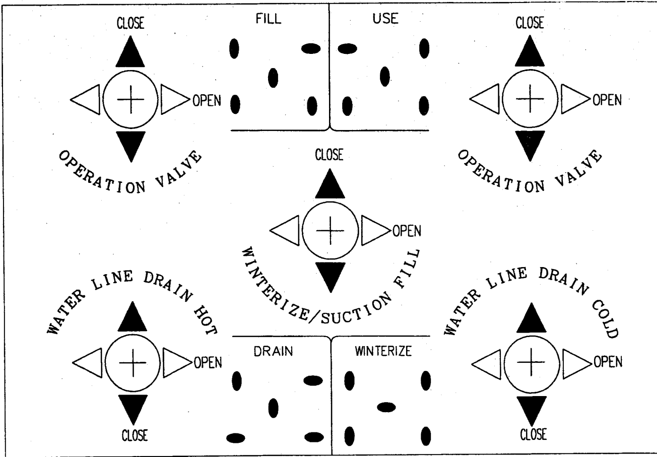
WATER CONTROL SYSTEM
