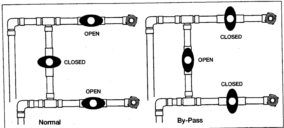
WATER HEATER BY-PASS (TYPICAL)
