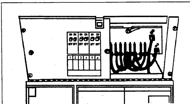
COMBINED POWER CENTER/CONVERTER
