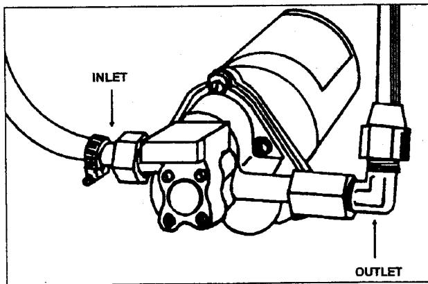
WATER PUMP
