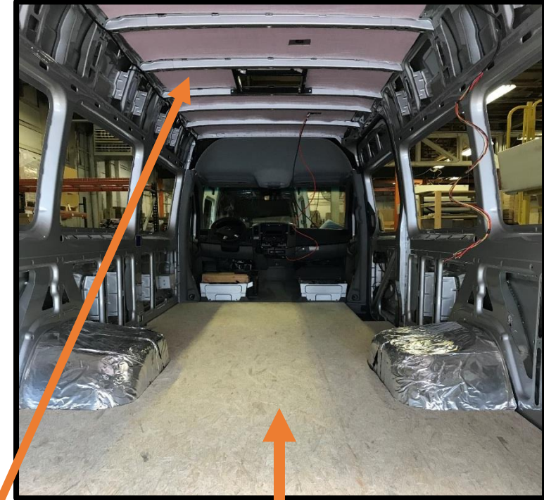
ONE PIECE 5/8" MARINE GRADE OSB FLOOR
