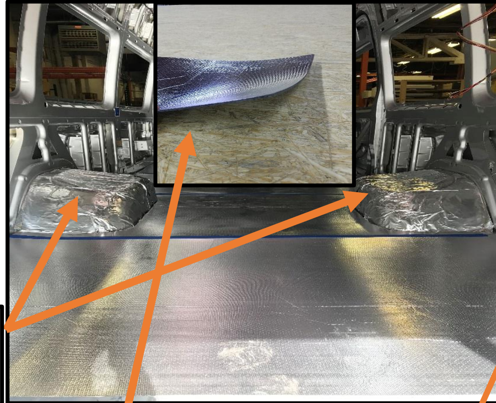
Kozy Wrap R-38 insulation and sound deadener
