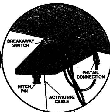
PIN BOX FIGURE 3
