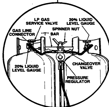
DUAL LP GAS BOTTLES FIGURE 16
