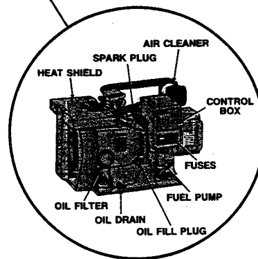
GENERATOR FIGURE 10
