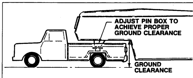
FIFTH WHEEL GROUND CLEARANCE
