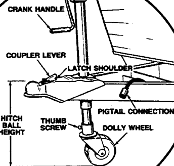
FRONT JACK FIGURE 1
