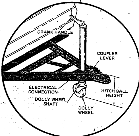
ELECTRIC BRAKE COUPLER FIGURE 1
