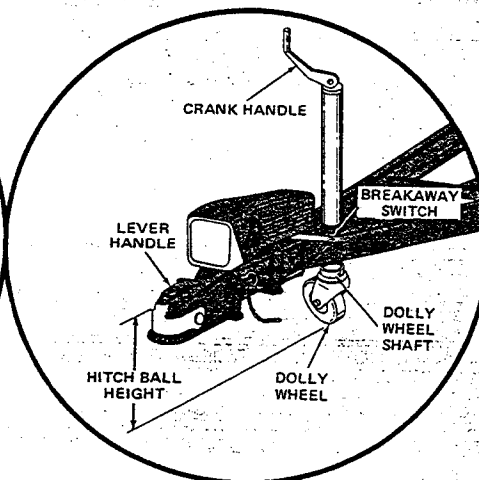
HYDRAULIC BRAKE COUPLER FIGURE 3
