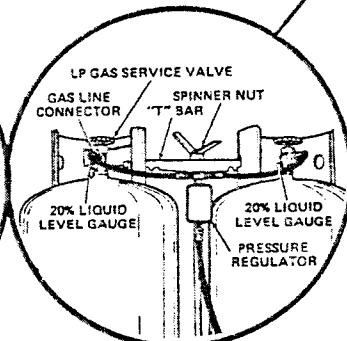
DUAL LP GAS BOTTLES FIGURE 18
