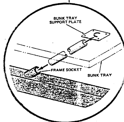
TRAILER FRAME BUNK SUPPORTS FIGURE 12
