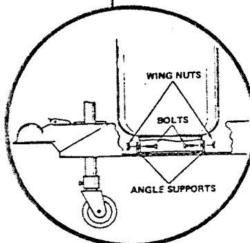
SINGLE LP GAS BOTTLE FIGURE 19
