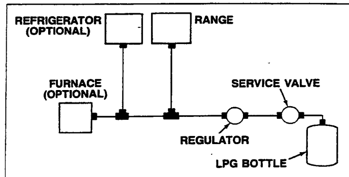
LP GAS SYSTEM (TYPICAL)
