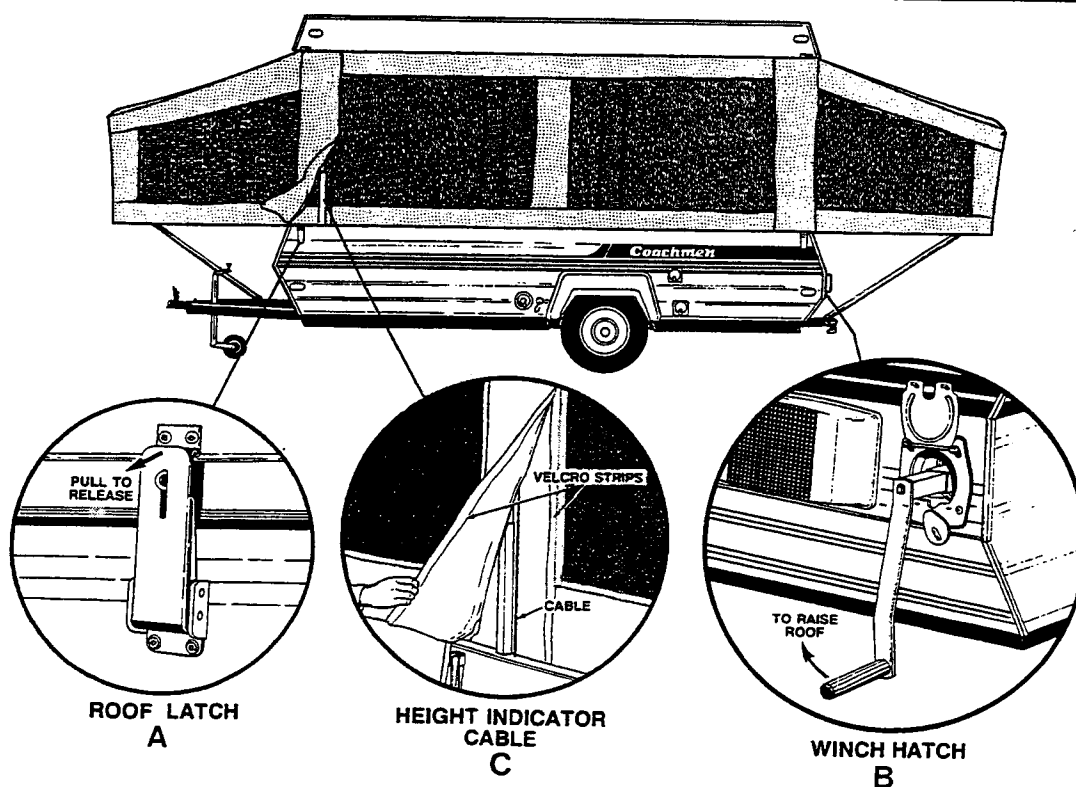
CRANK LIFT SYSTEM
