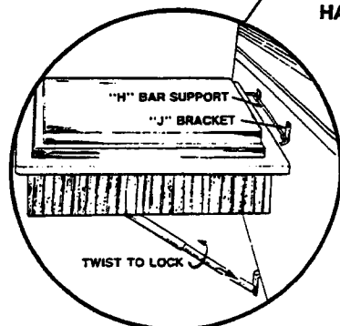
OUTDOOR STOVE SET-UP FIGURE 7
