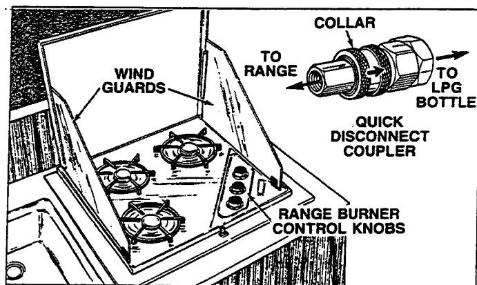
INSIDE/OUTSIDE STOVE
