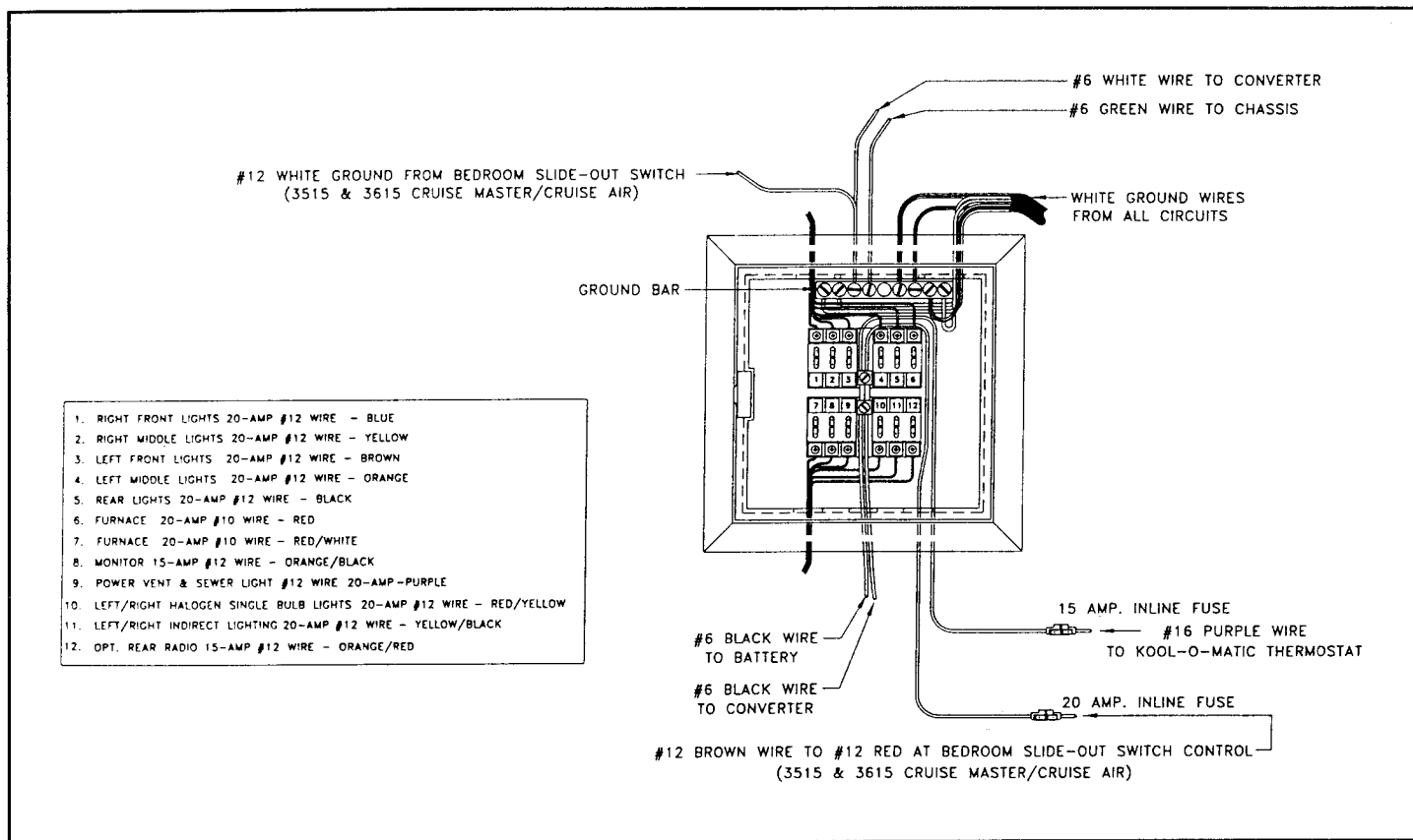
Typical 12-Volt 12-Circuit Power Converter Fuse Panel (CSA)
