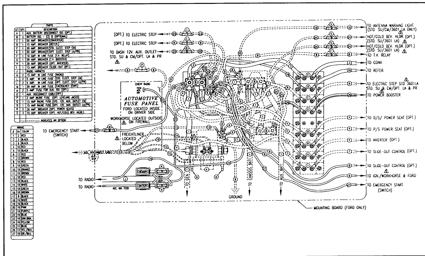
Typical Automotive Electric Circuit (Workhorse)
