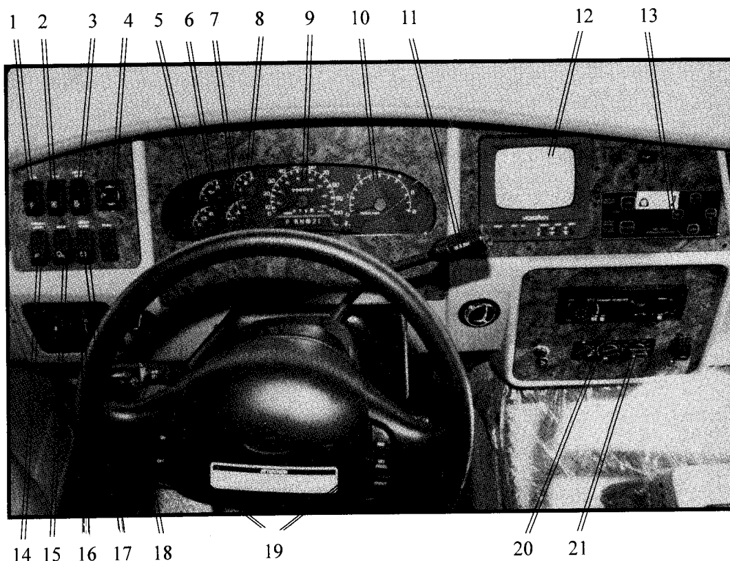
Cruise Air Driver's Compartment (Ford)
