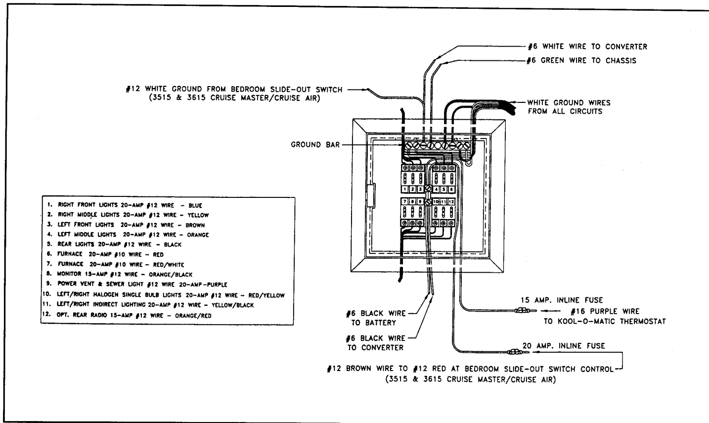
Typical 12-Volt 12-Circuit Power Converter Fuse Panel (All Models)
