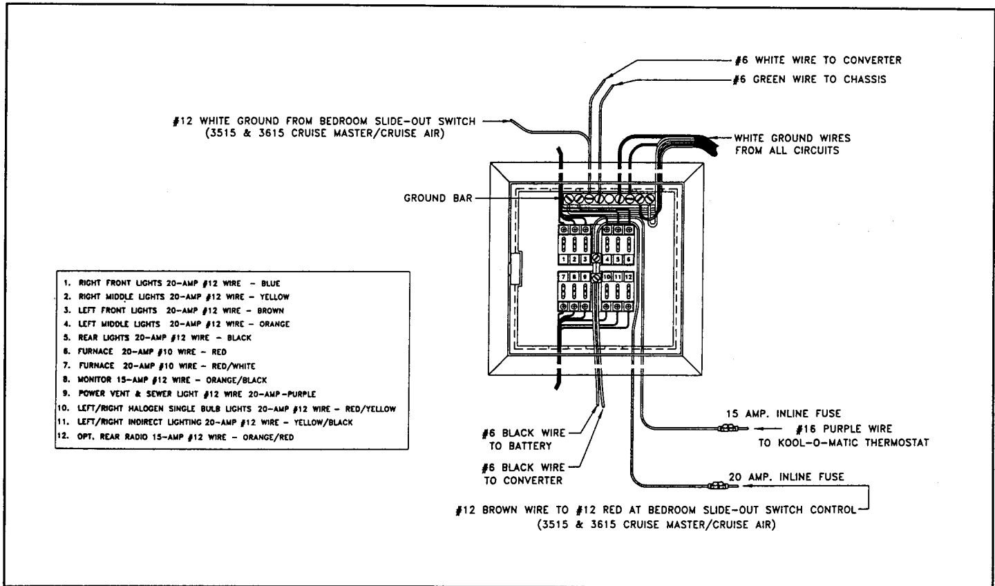
Typical 12-Volt 12-Circuit Power Converter Fuse Panel (All Models)
