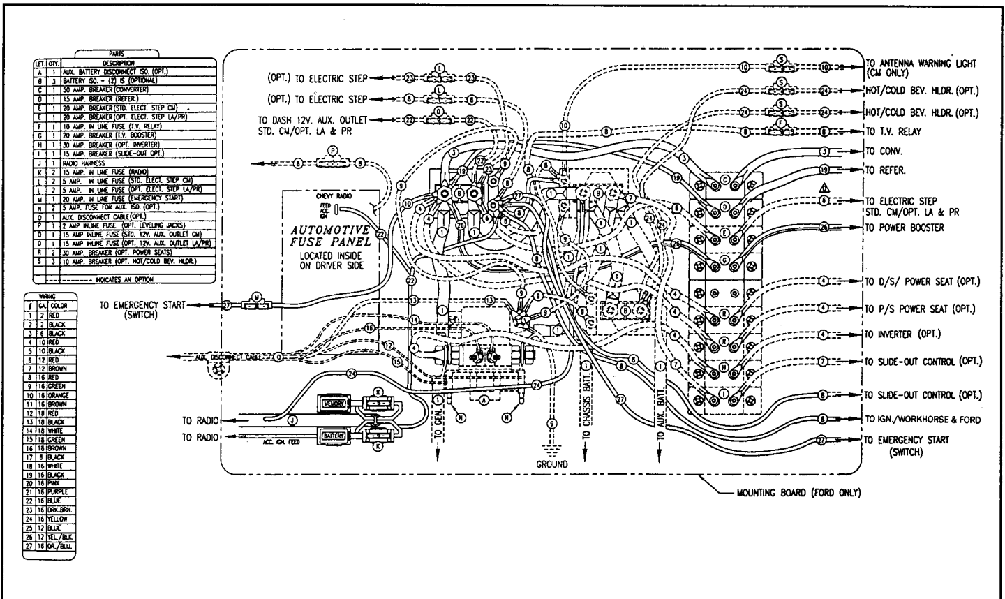
Typical Automotive Electric Circuit (Workhorse and Ford)
