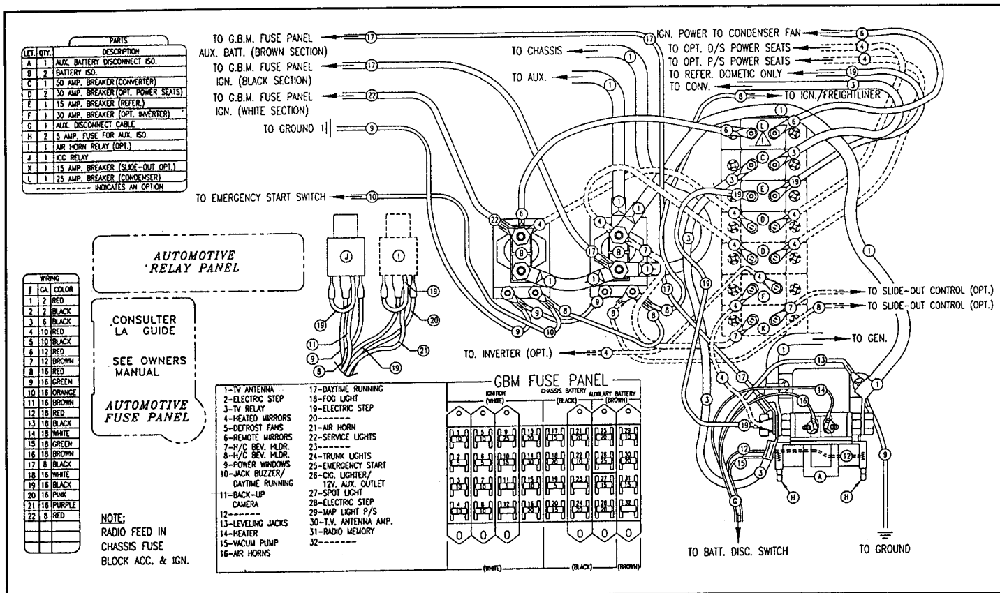
Typical Automotive Electric Circuit (Freightliner)
