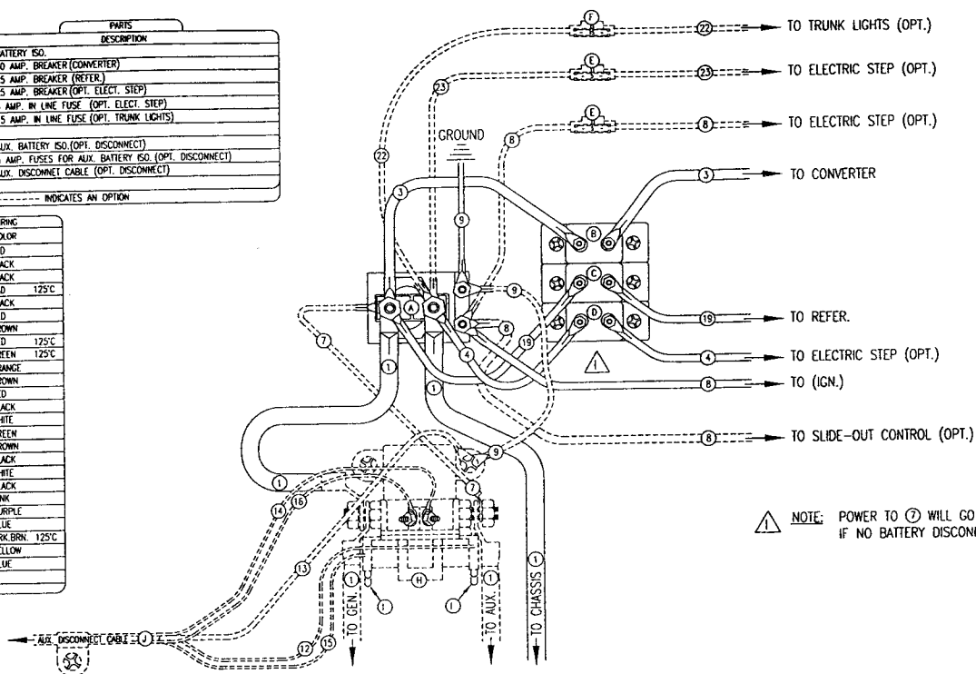
Typical Automotive Electrical Circuit (Ford)
