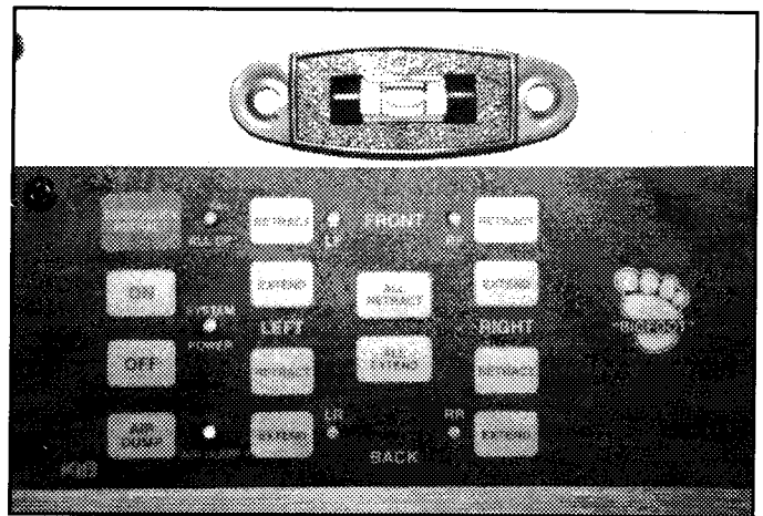
Typical Jack Controls
