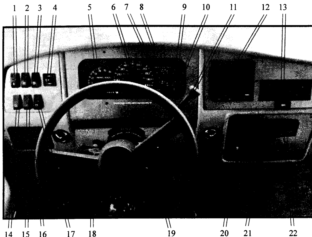
Cruise Master Driver's Compartment (Chevy)
