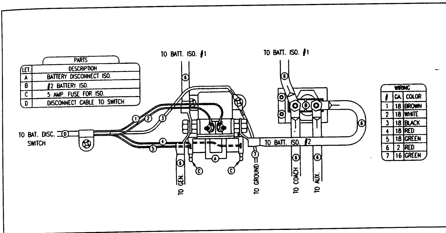
Typical Auxiliary Battery Disconnect Circuit
