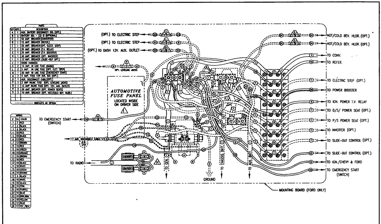
Typical Automotive Electric Circuit (Chevy and Ford)
