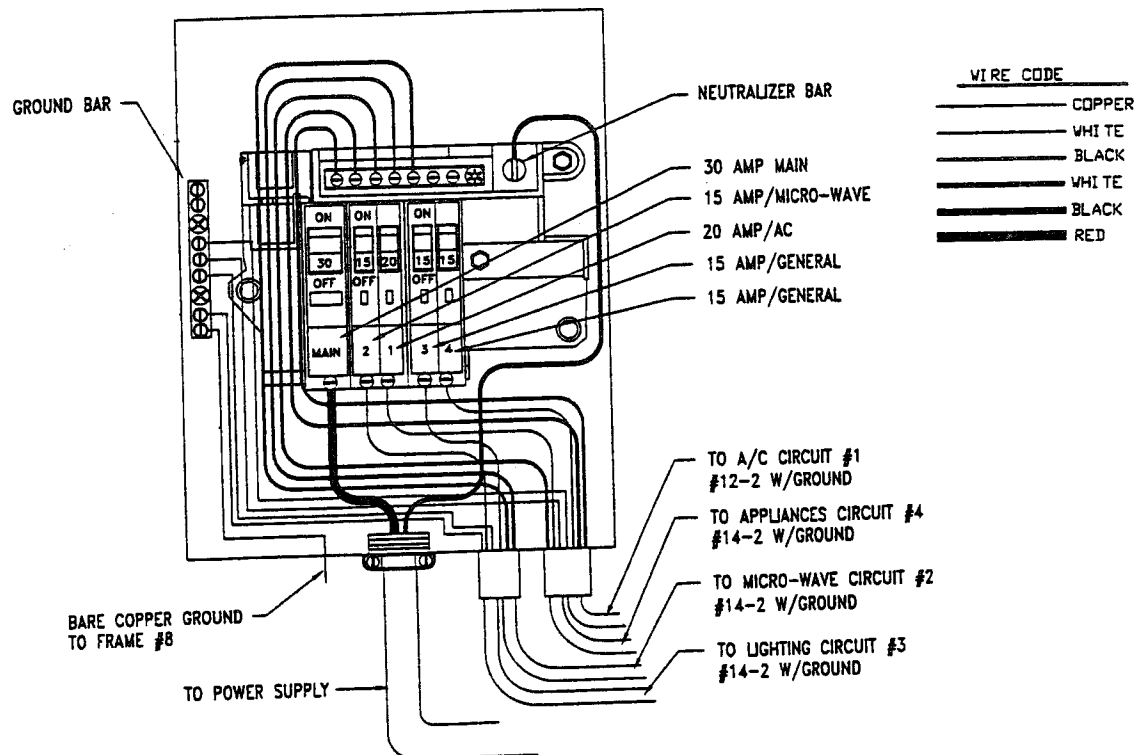
Typical 120-Volt 30-Amp Electrical Circuit
