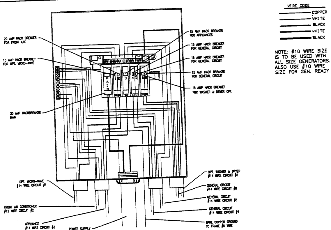
Typical 120-Volt 30-Amp Electrical Circuit (CSA)
