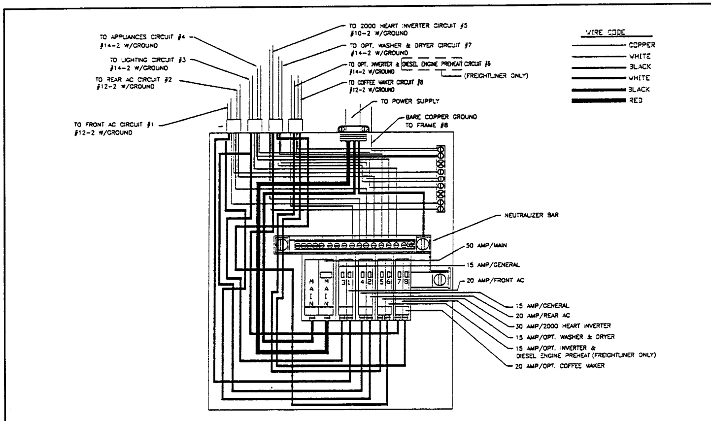
Typical 120-Volt 50-Amp Electrical Circuit with 2000 Heart Inverter
