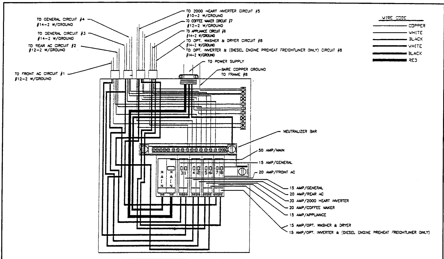
Typical 120-Volt 50-Amp Electrical Circuit with the 2000 Heart Inverter (CSA)
