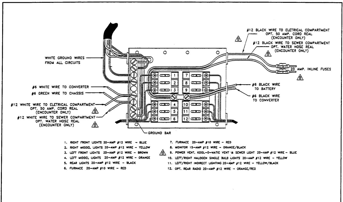
Typical 12-Volt & 12-Volt (CSA) Power Converter Fuse Panel
