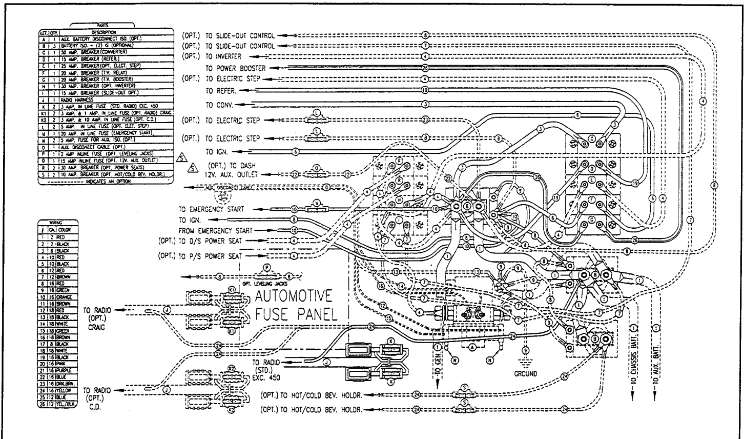
Typical Automotive Electric Circuit (Chevy)
