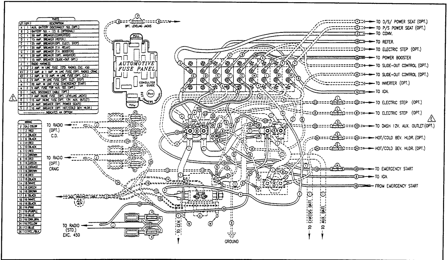
Typical Automotive Electric Circuit (Ford)
