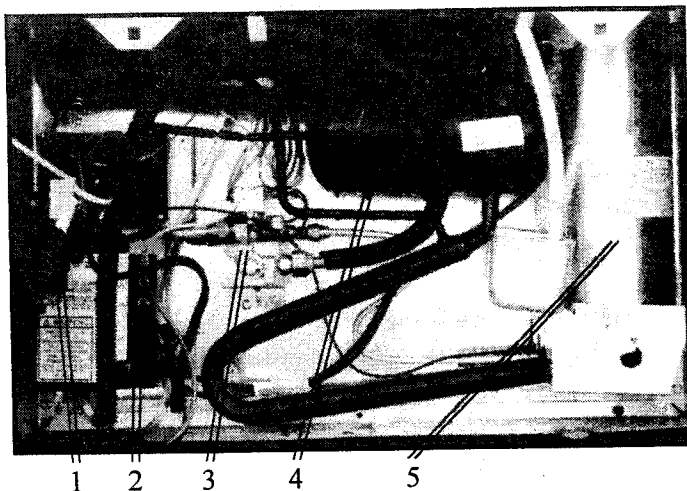
Refrigerator Vent
