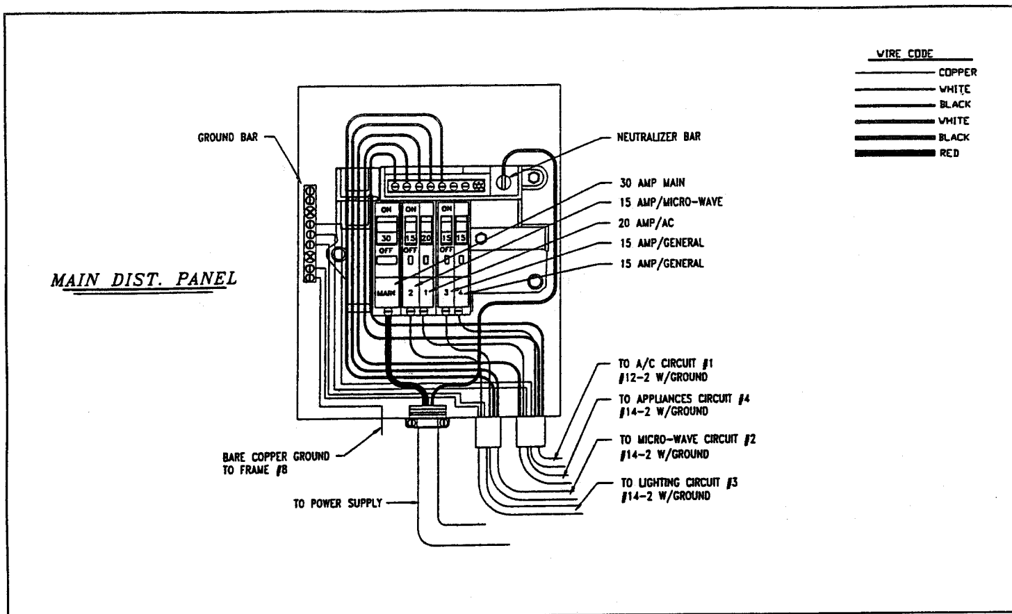
Typical 120-Volt 30-Amp Electrical Circuit
