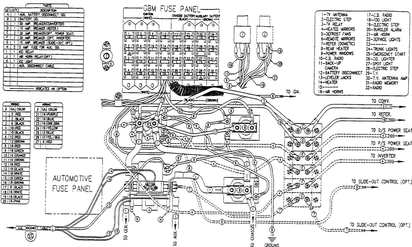
Typical Automotive Electric Circuit for Cruise Air (Chevy and Ford Chassis 1996)
