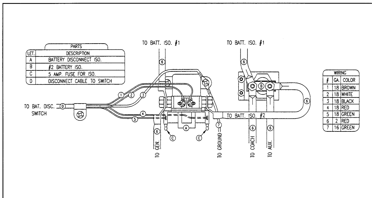
Auxiliary Battery Disconnect Circuit
