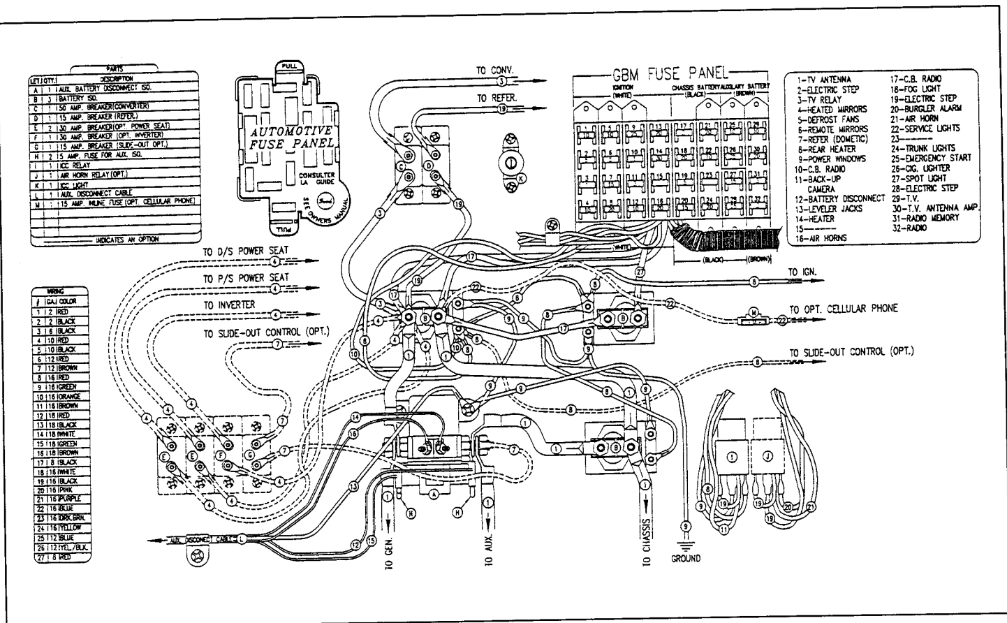
Typical automotive Electric Circuit for Cruise Air (Ford 1997)
