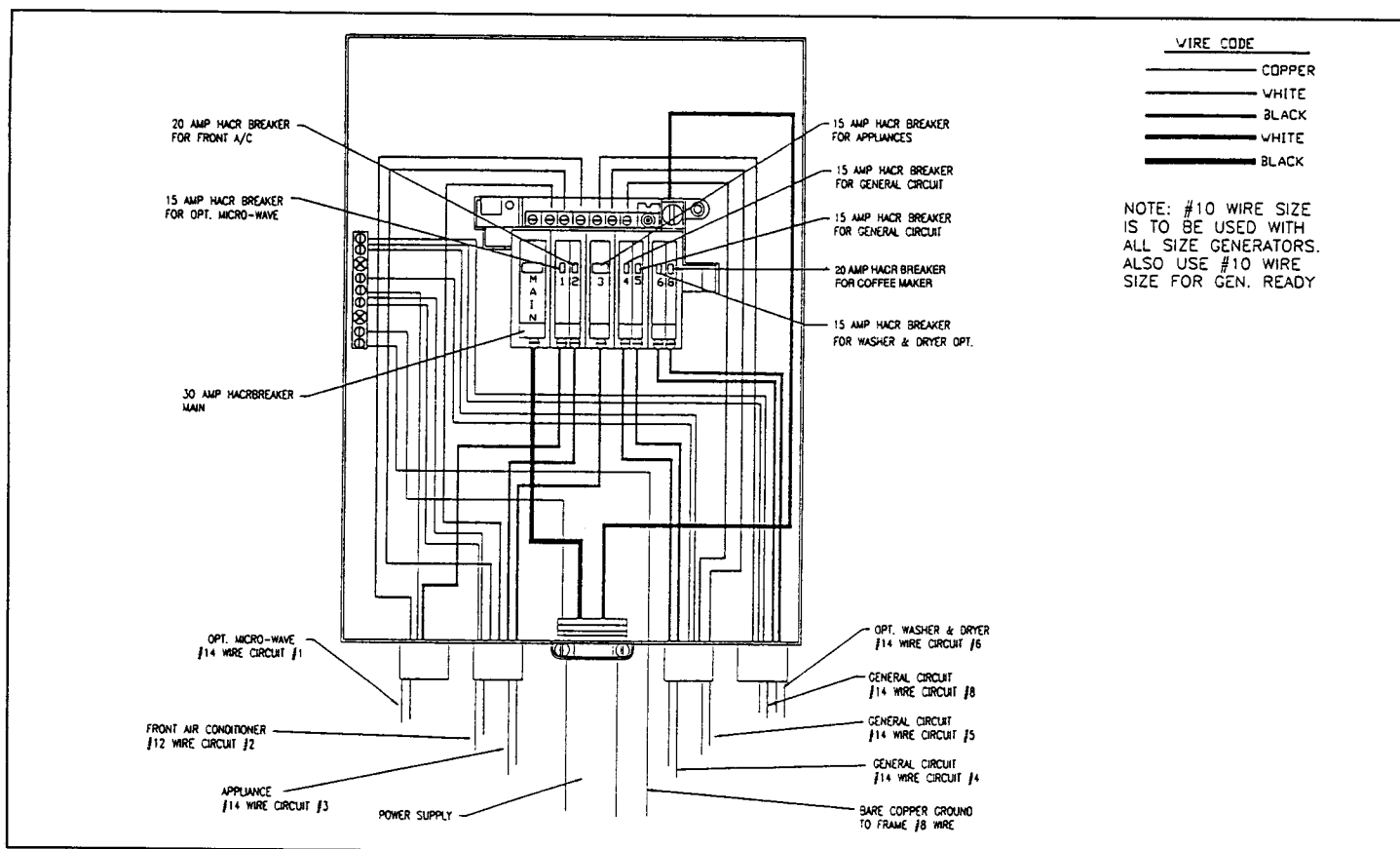
Typical 120-Volt 30-Amp Electrical System (CSA)
