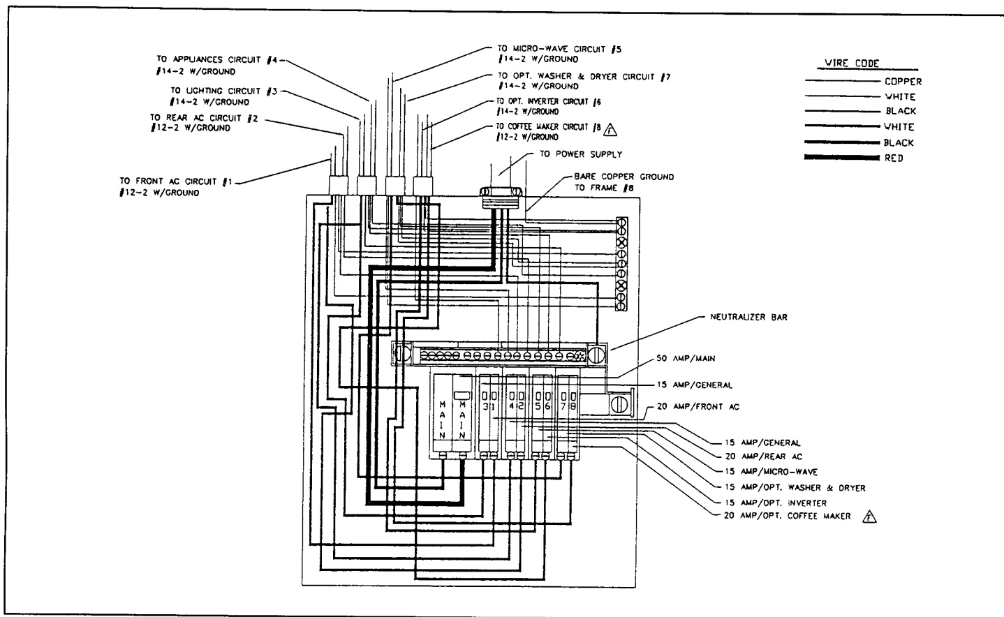
Typical 120-Volt 50-Amp Electrical System
