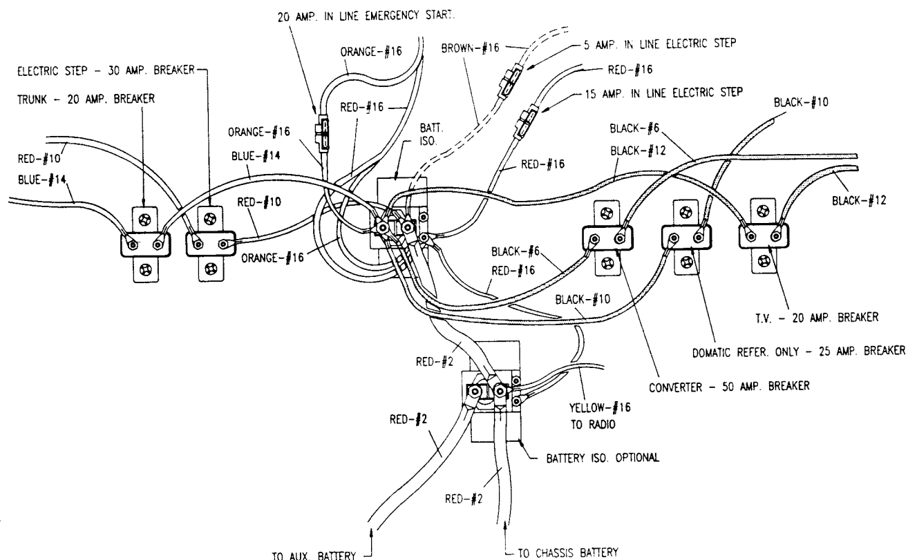
Typical Automotive Electric Circuit
