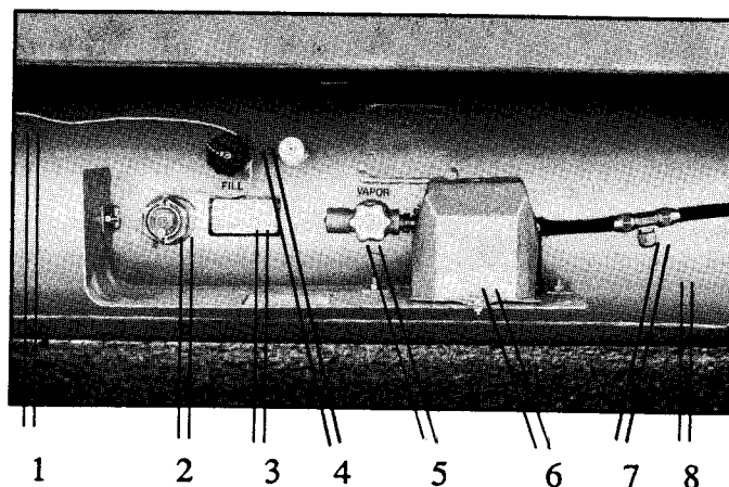
Typical Liquid Petroleum Gas Tank
