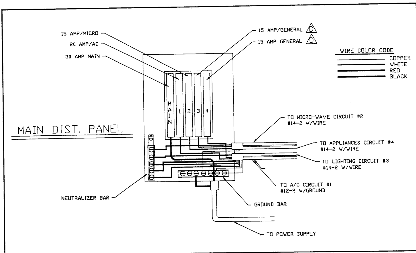
Typical 115-Volt 30-Amp Electrical Circuit
