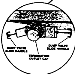
TERMINATION OUTLET
