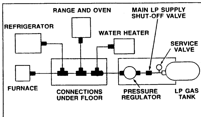
LP GAS SYSTEM (TYPICAL)
