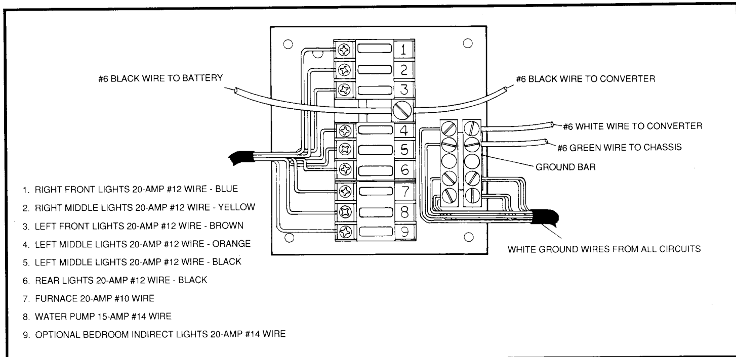
Typical 12-Volt Power Converter Fuse Panel For Cruise Air III and Cruise Master Models 30', 32', 34', and 36'
