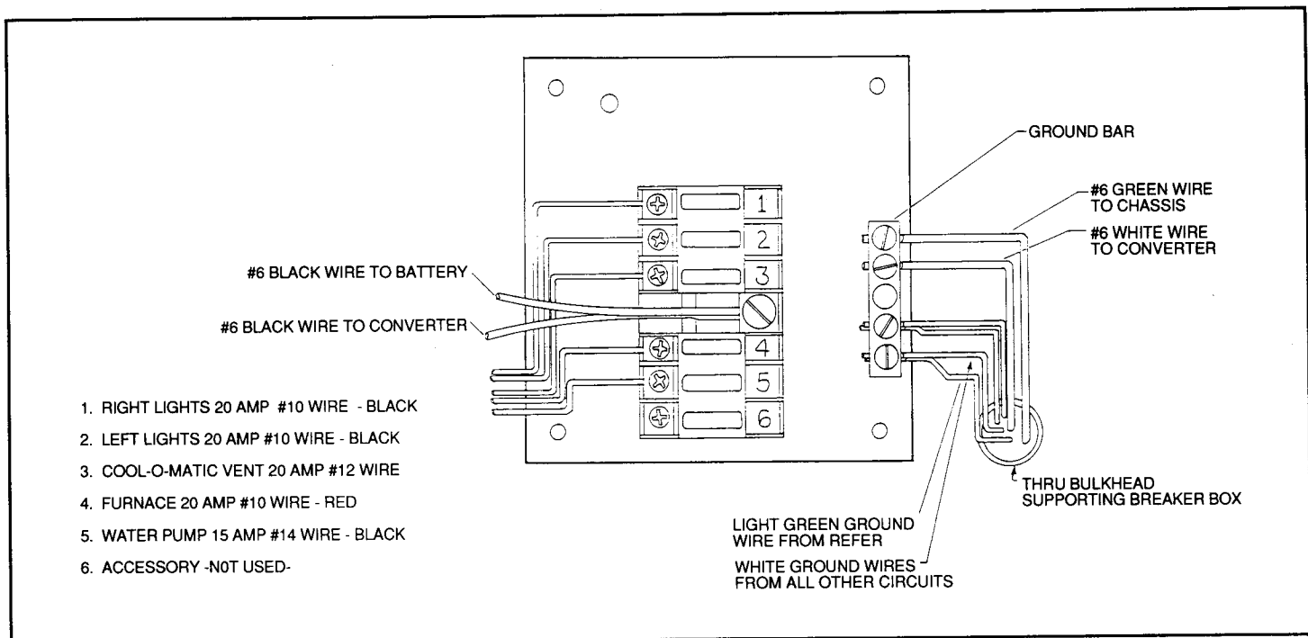
Typical 12-Volt Power Converter Fuse Panel For Cruise Master Model 28'
