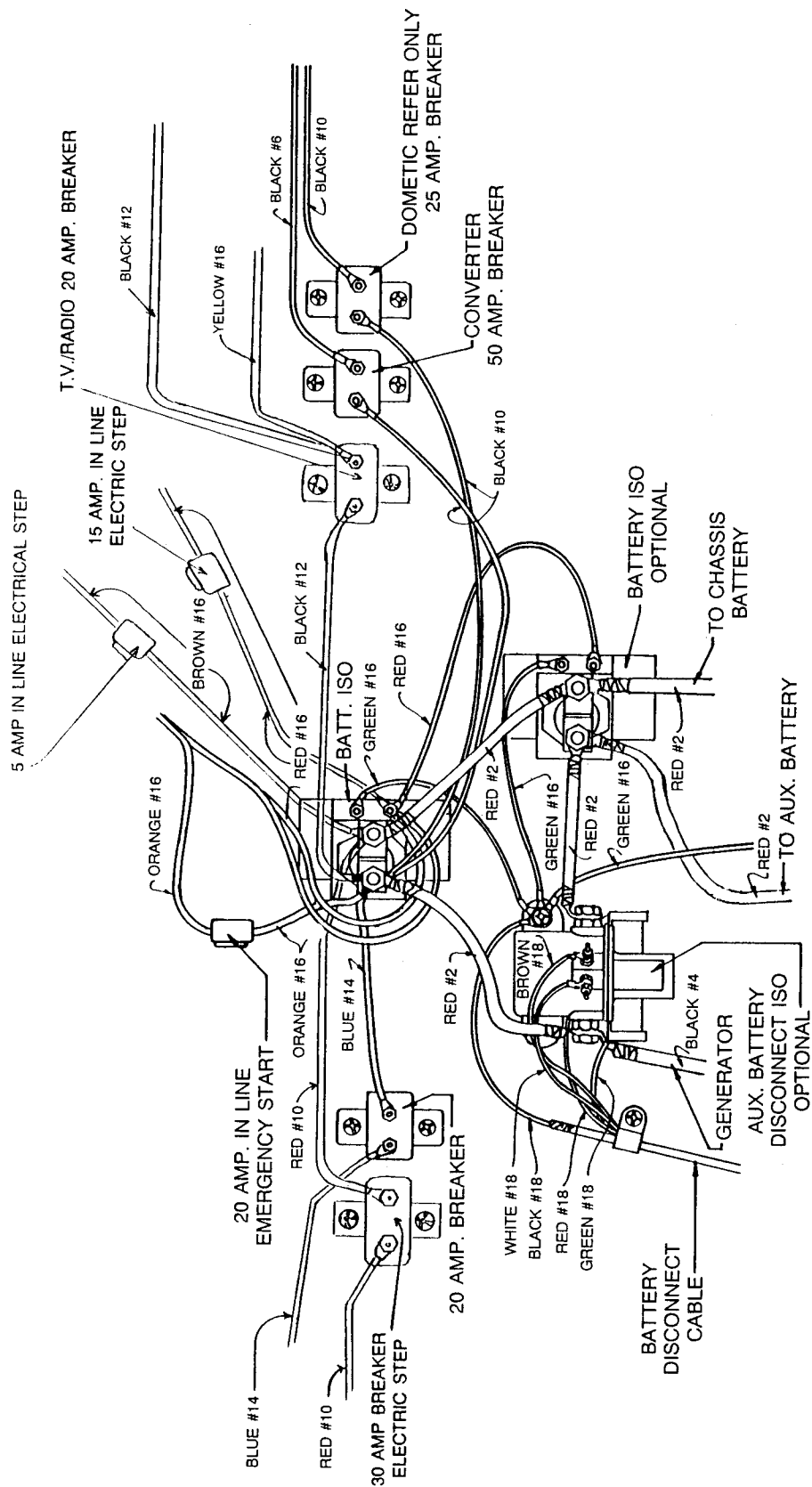
Typical Automotive Electrical Circuit for Cruise Master
