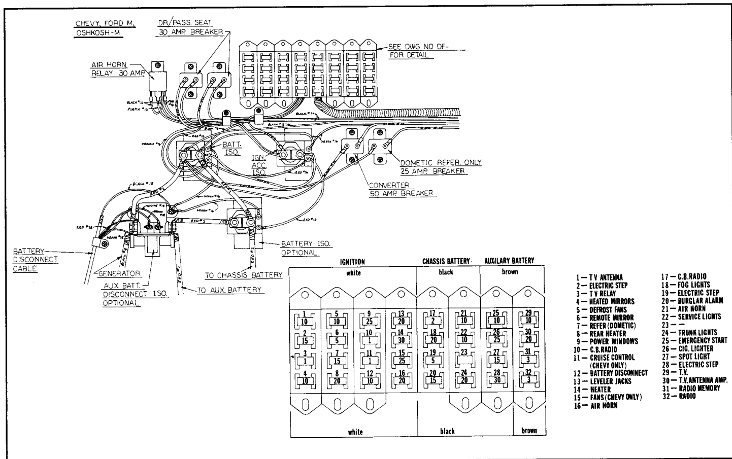
Typical Automotive Electrical Circuit for Cruise Air III
