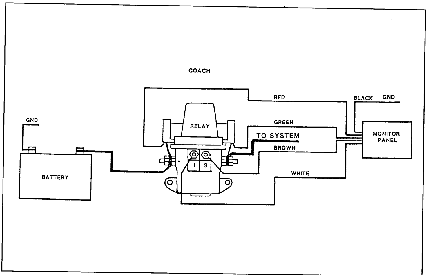
Auxiliary Battery Disconnect Circuit on Impulse and Encounter
