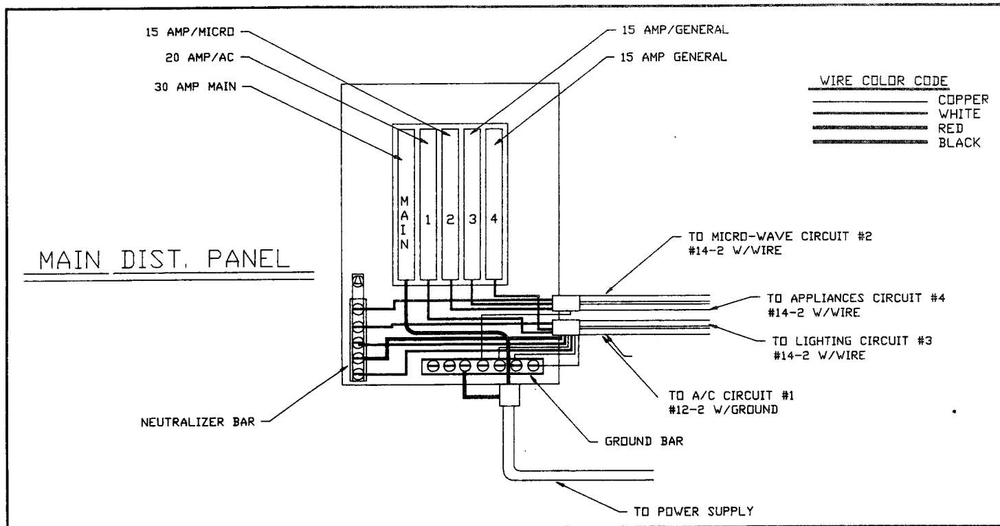
Typical 115-Volt 30-Amp Electrical Circuit
