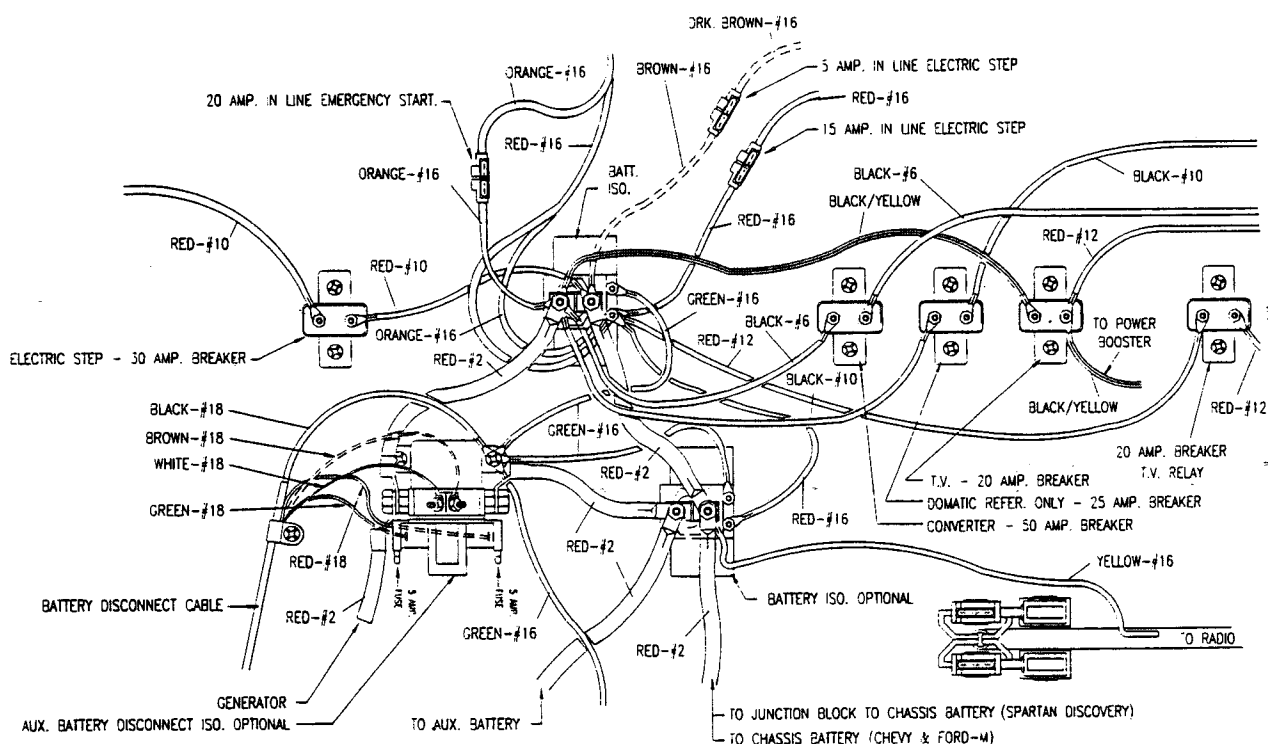
Typical Automotive Electric Circuit
