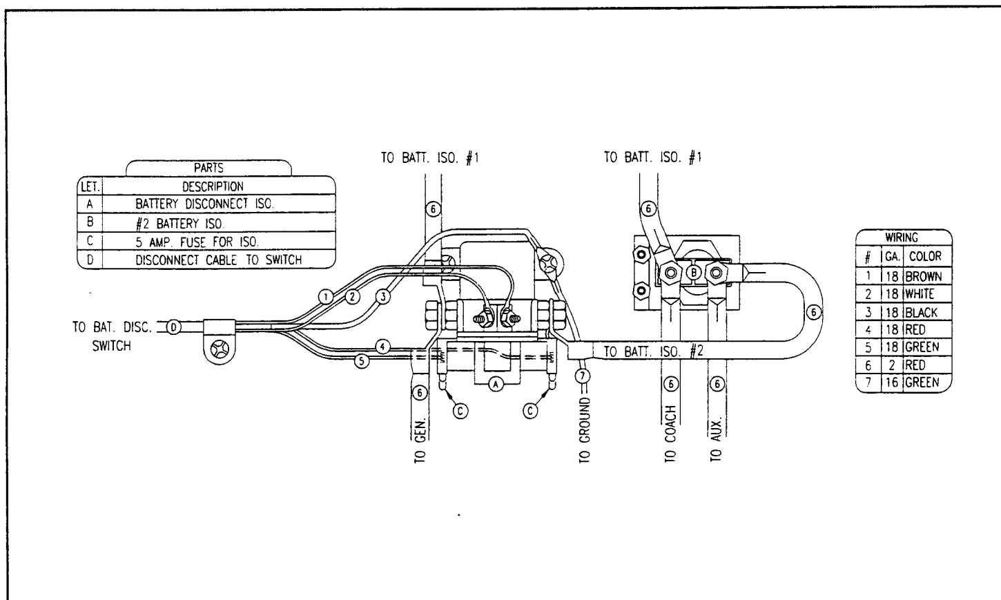
Typical Auxiliary Battery Disconnect Circuit
