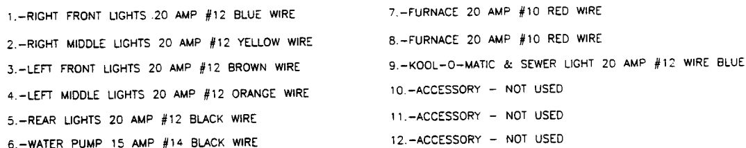
Typical 12-Volt 12-Circuit Power Converter Fuse Panel (CSA)
