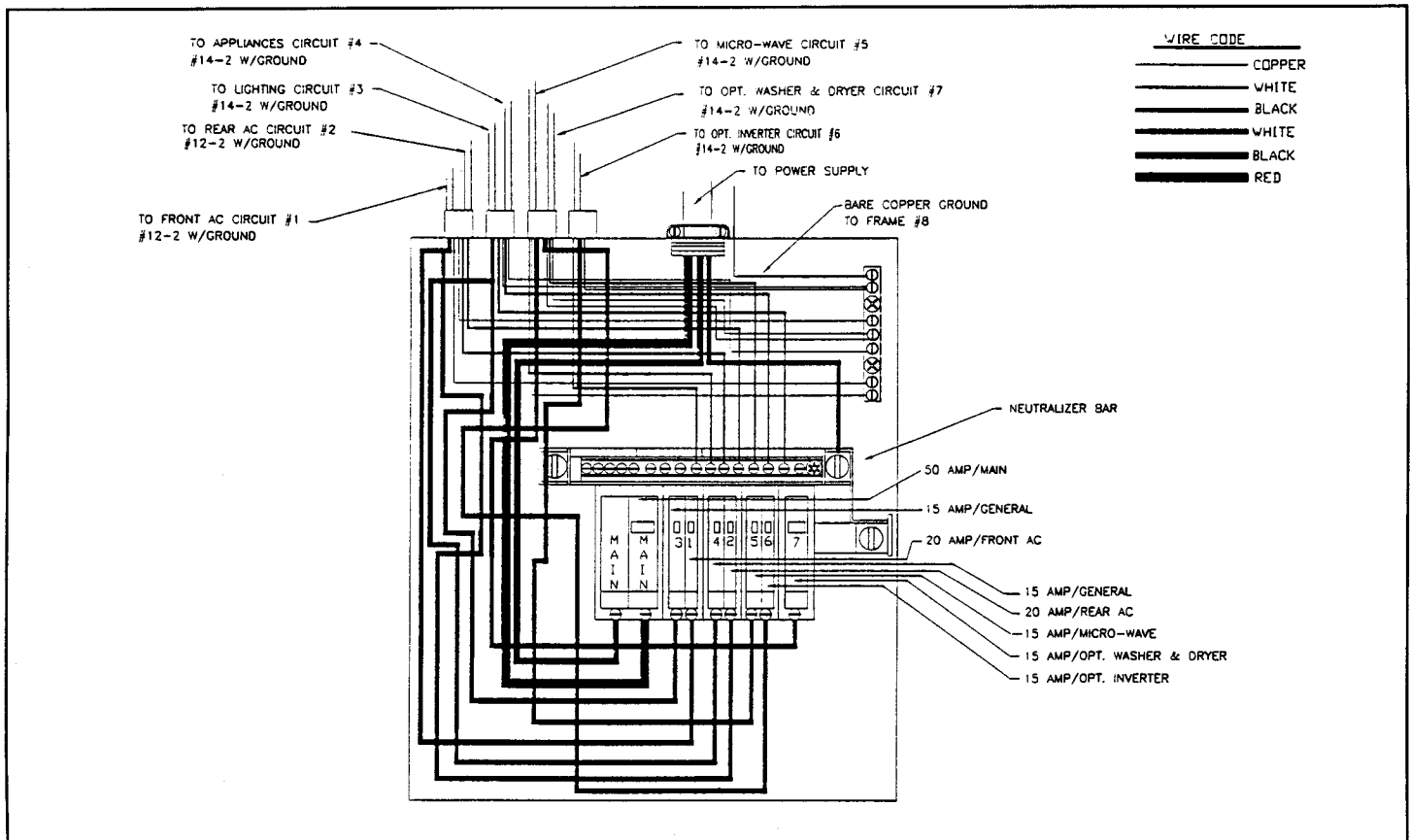
Typical 120-Volt 50-Amp Electrical System
