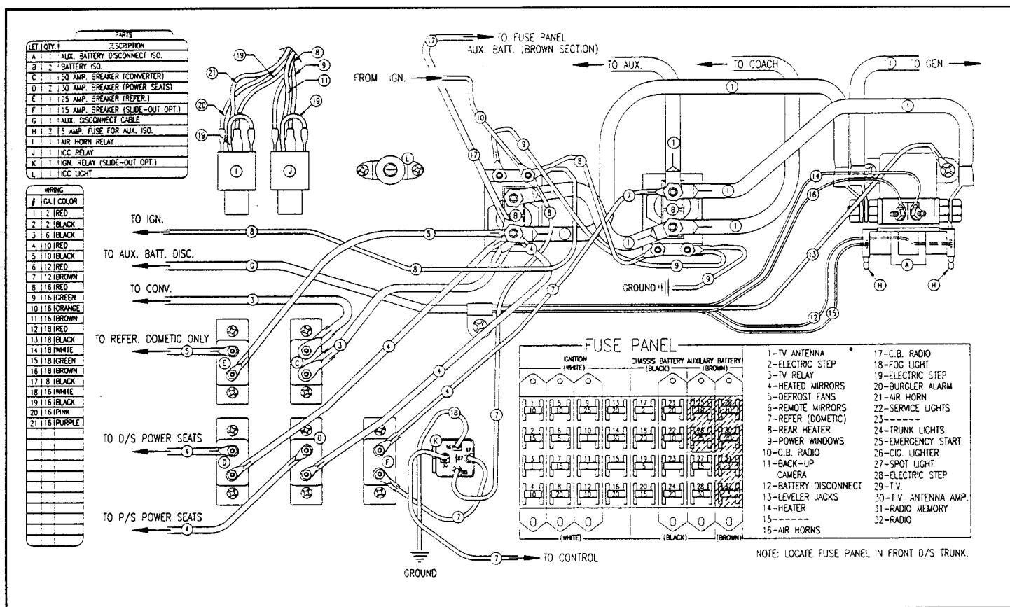
Typical Automotive Electric Circuit for Spartan
