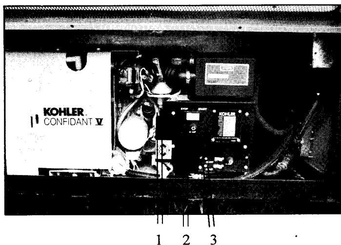
Typical Cruise Air and Encounter Generator (Driver's side of motor home)
