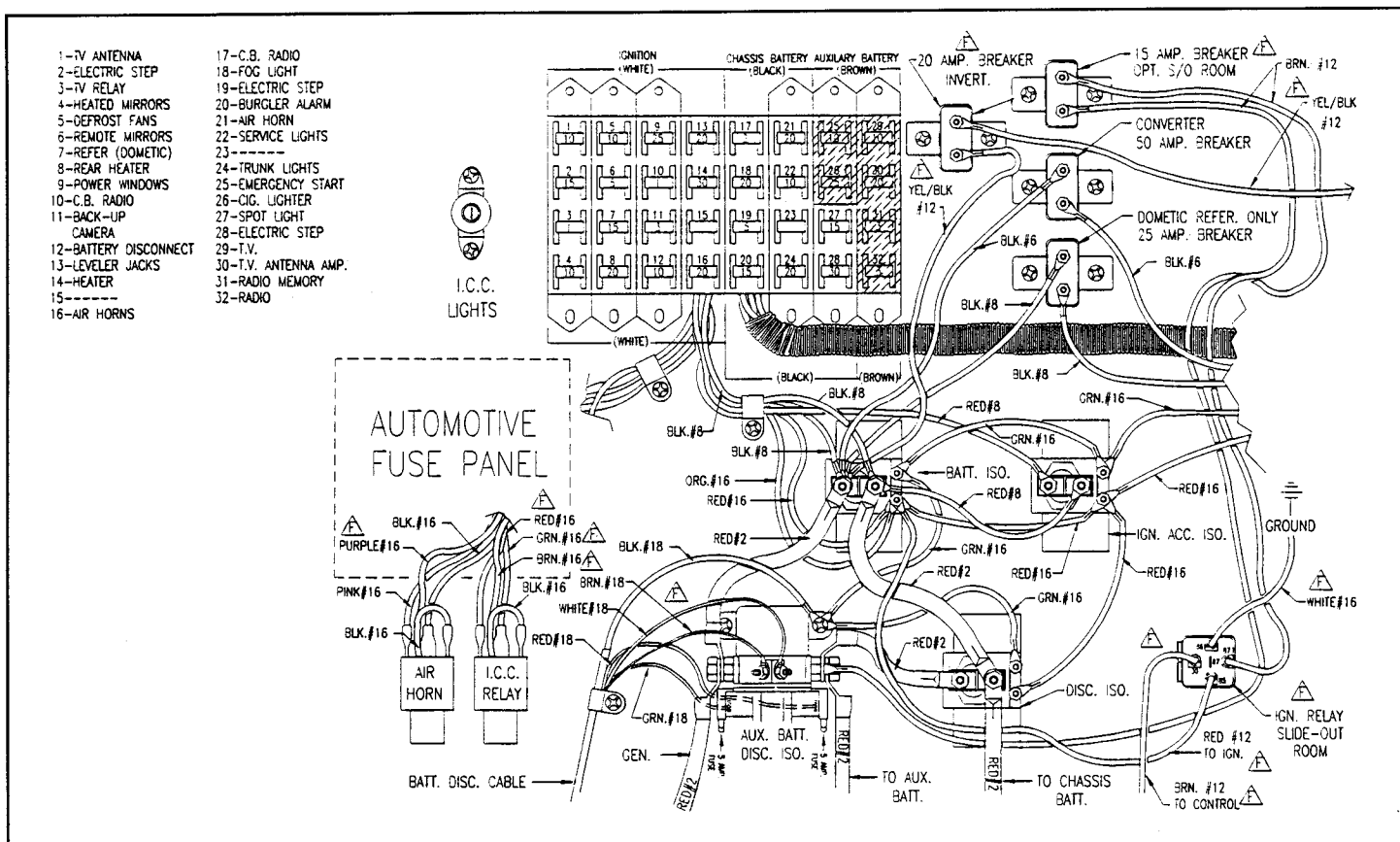
Typical Automotive Electric Circuit for Encounter and Cruise Air (Chevy and Ford)
