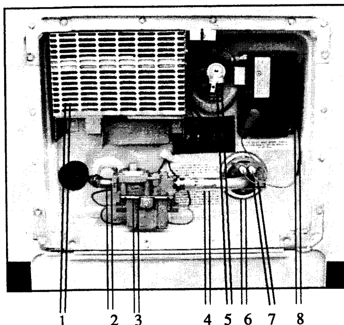
Water Heater
