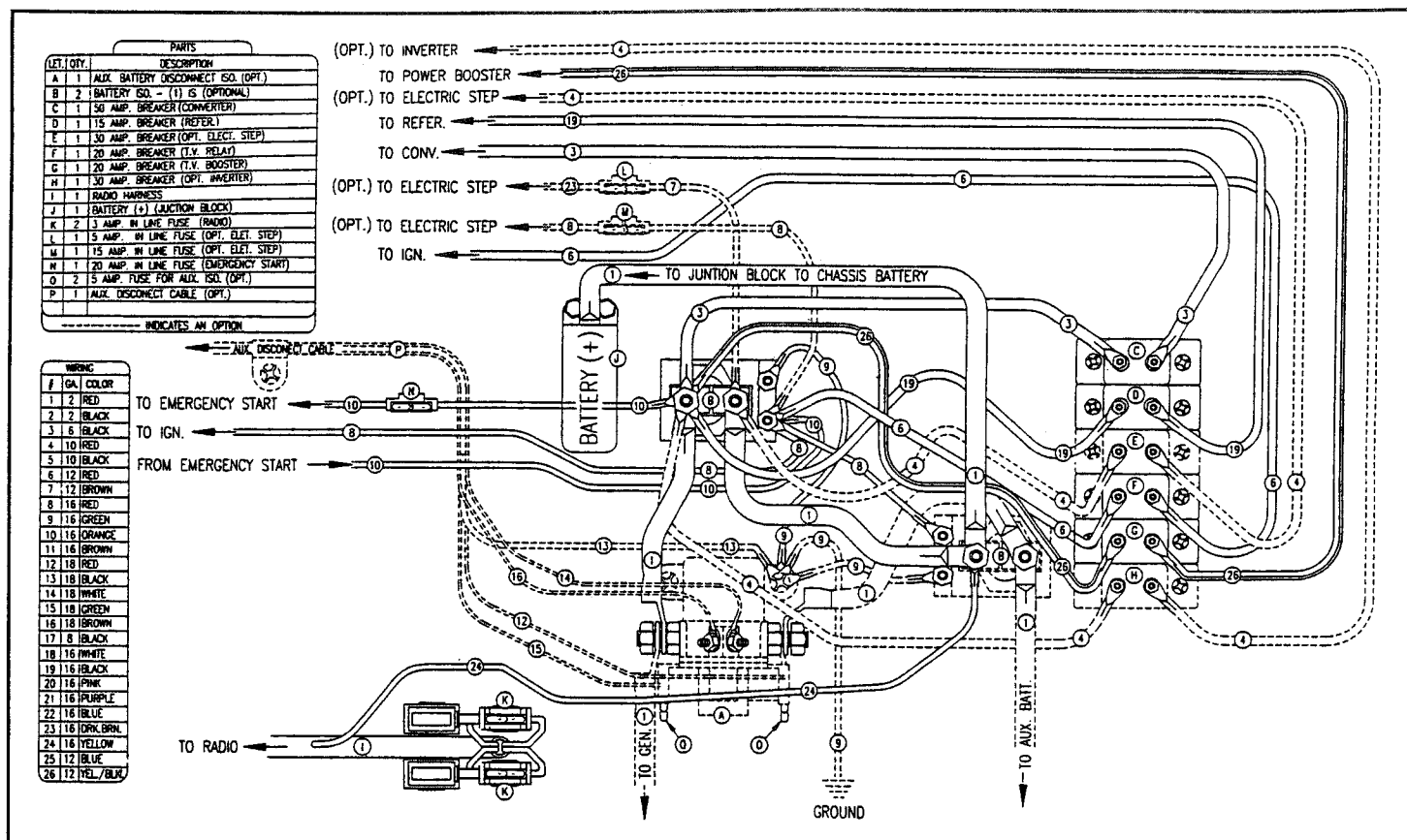
Typical Automotive Electric Circuit (Spartan Discovery Models)
