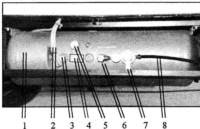
Typical Liquid Petroleum Tank
