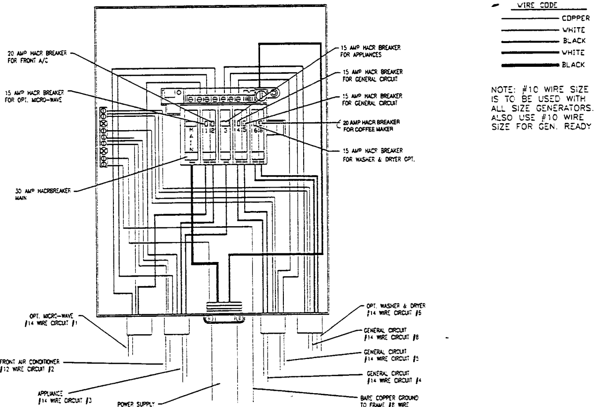
Typical 120-Volt 30-Amp Electrical Circuit (CSA)
