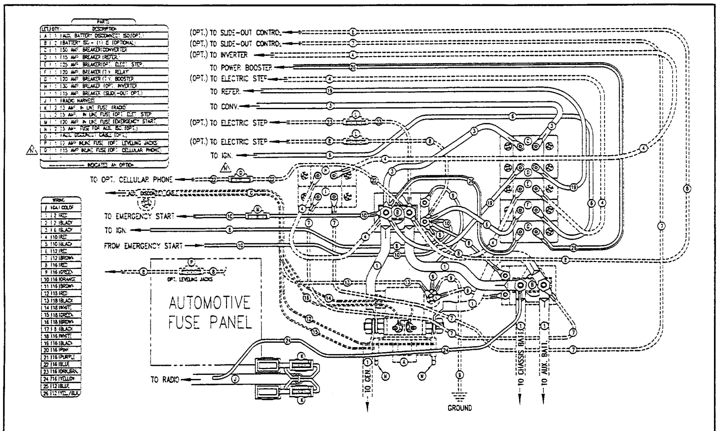
Typical Automotive Electric Circuit (Chevrolet and Ford)
