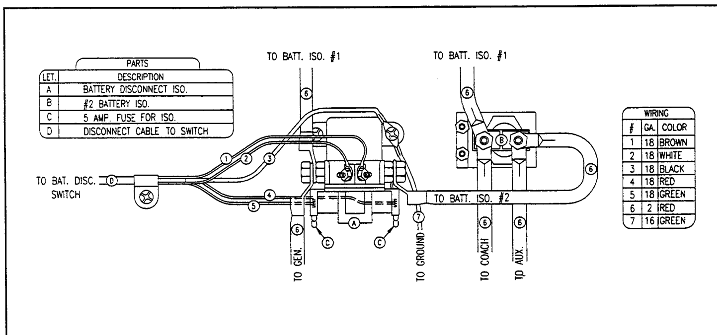
Typical Auxiliary Battery Disconnect Circuit
