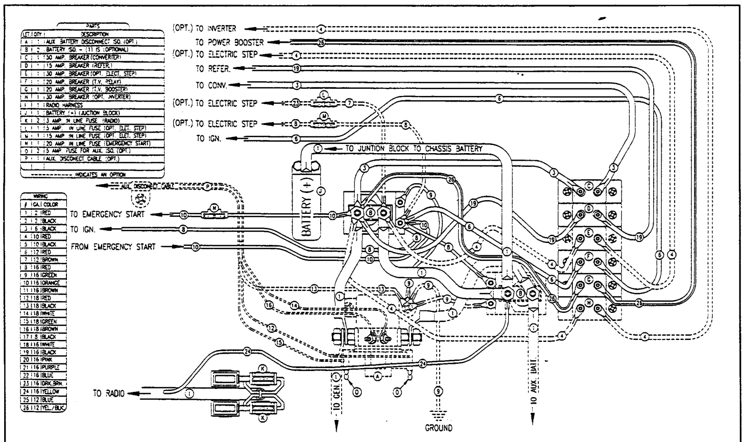
Typical Automotive Electric Circuit (Spartan Model)
