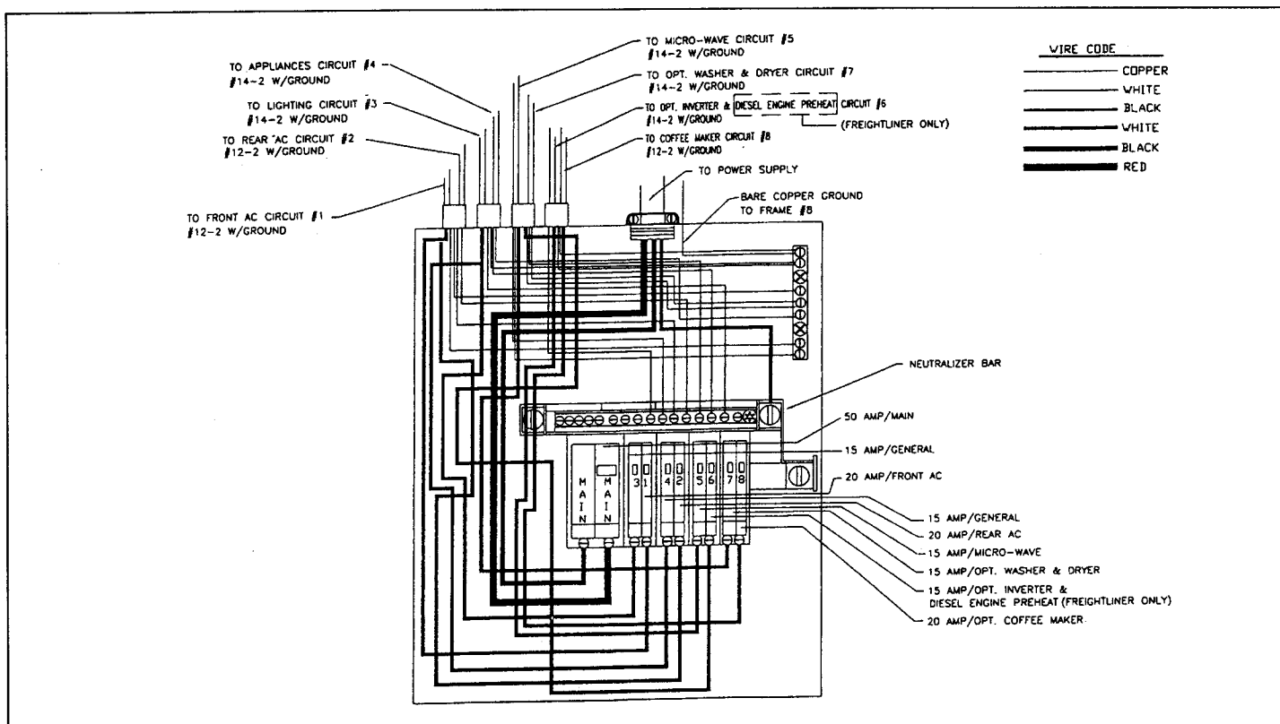
Typical 120-Volt 50-Amp Electrical Circuit
