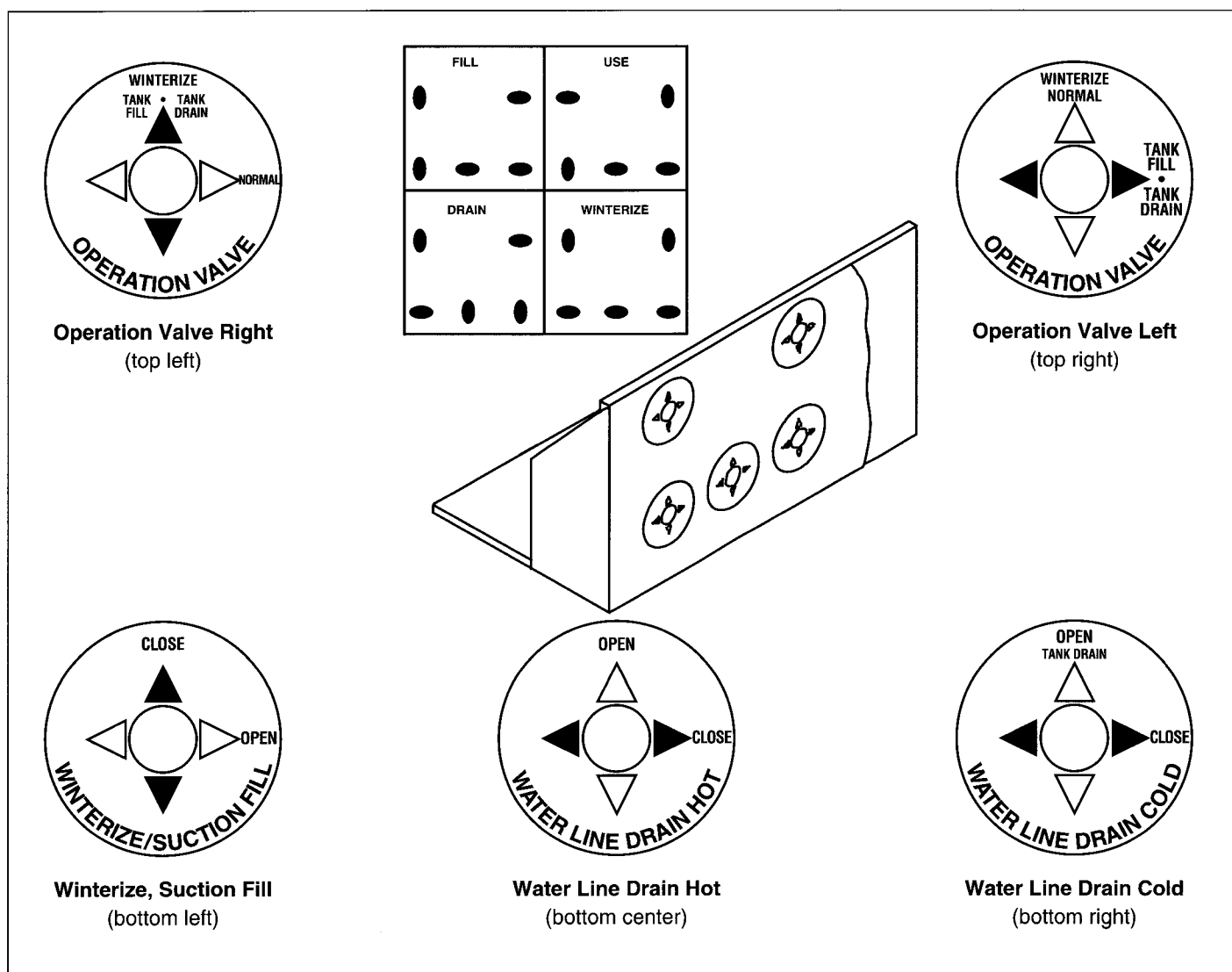
WATER VALVE CONTROL PANEL
