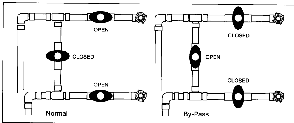
WATER HEATER BY-PASS (TYPICAL)
