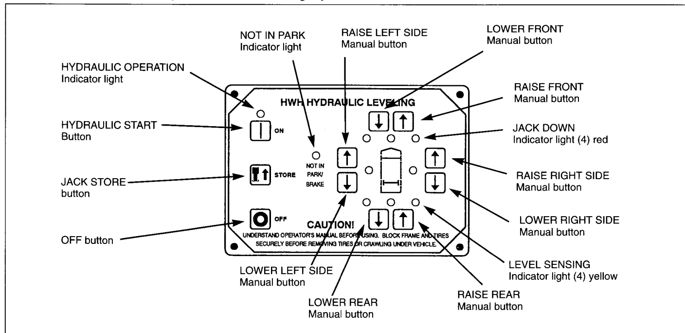
HYDRAULIC LEVELER PANEL
