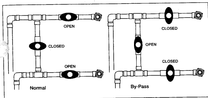
WATER HEATER BY-PASS (TYPICAL)
