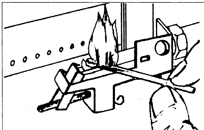
LIGHTING OVEN PILOT (when pilot is located on the right side of burner.)
