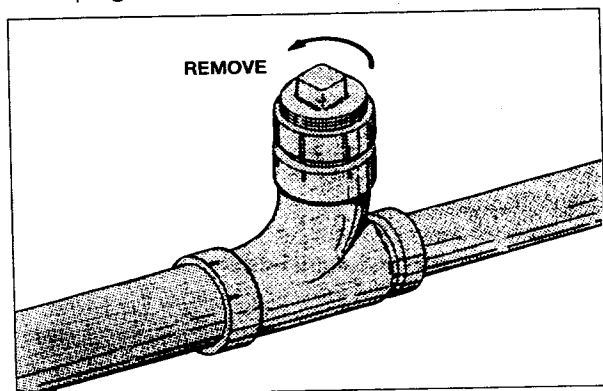
DRAIN CLEANOUT
