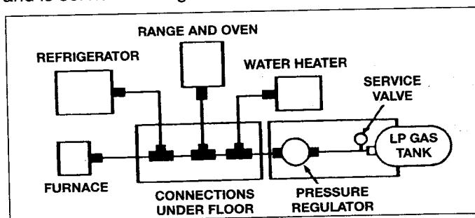
LP GAS SYSTEM (TYPICAL)
