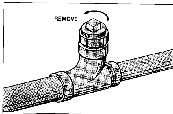
DRAIN CLEANOUT
