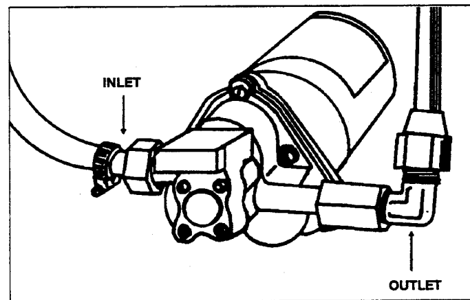
WATER PUMP
