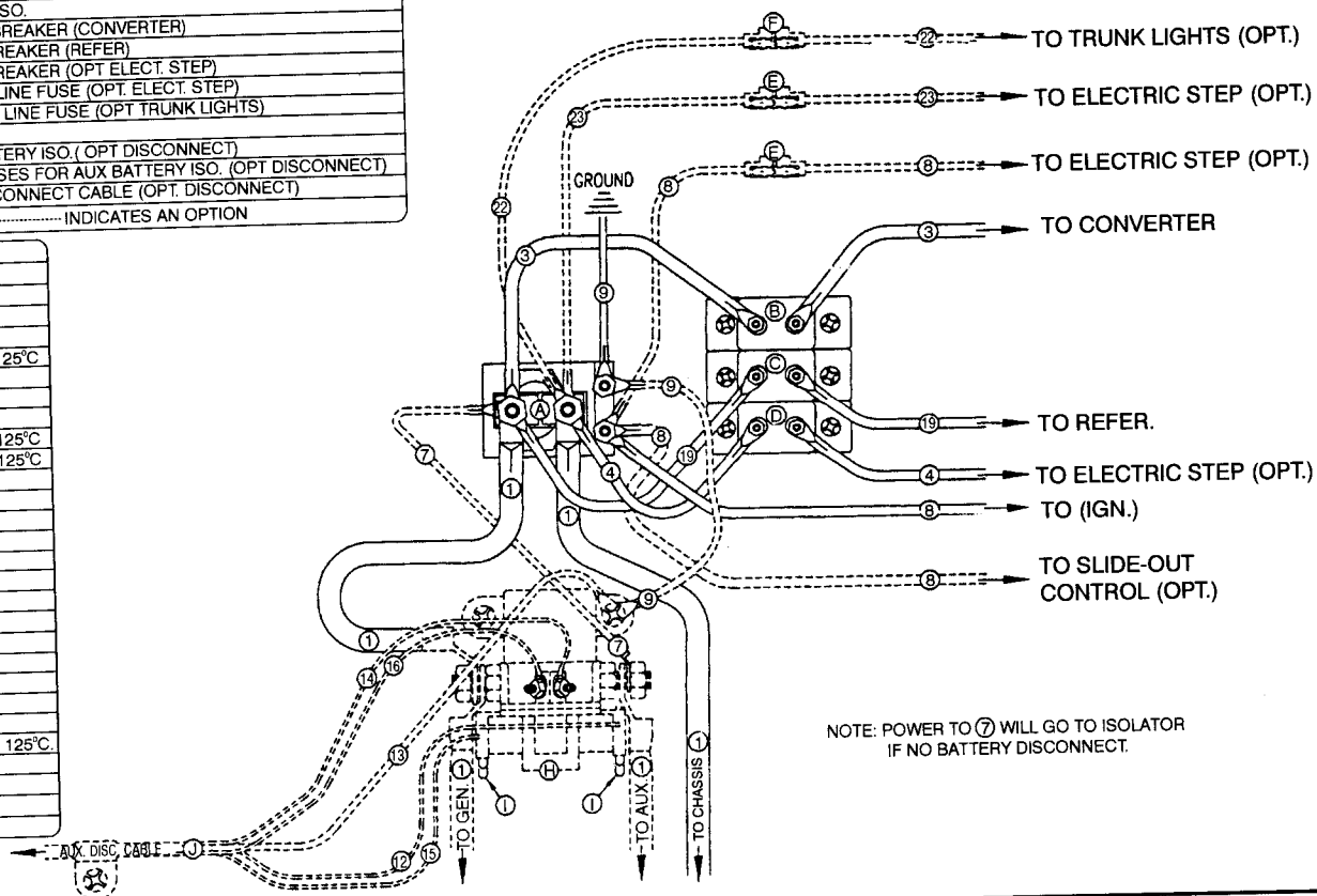
Typical Automotive Electrical Circuit
