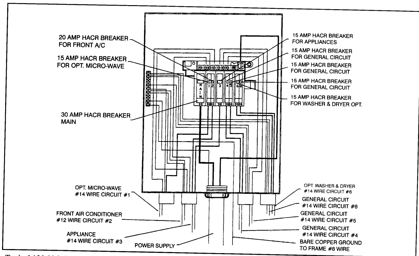
Typical 120-Volt 30-Amp Electrical Circuit (CSA)
