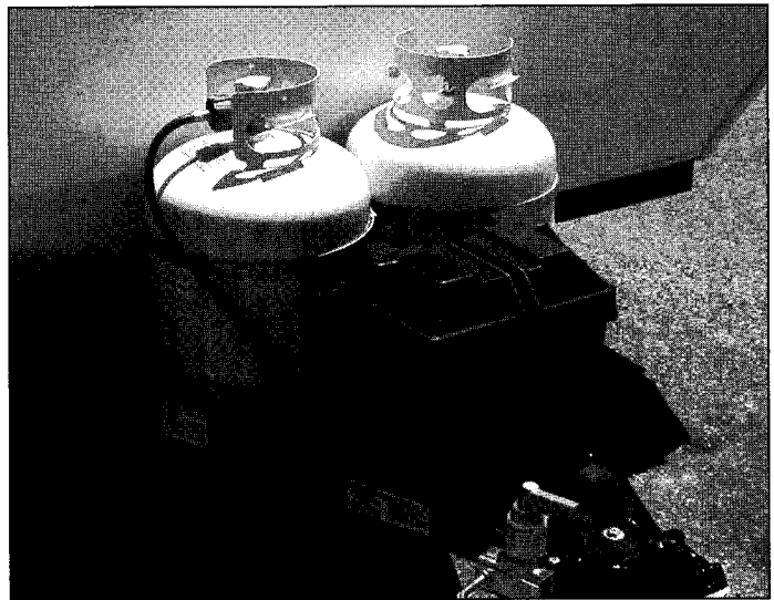
LPG HOSE ROUTING
