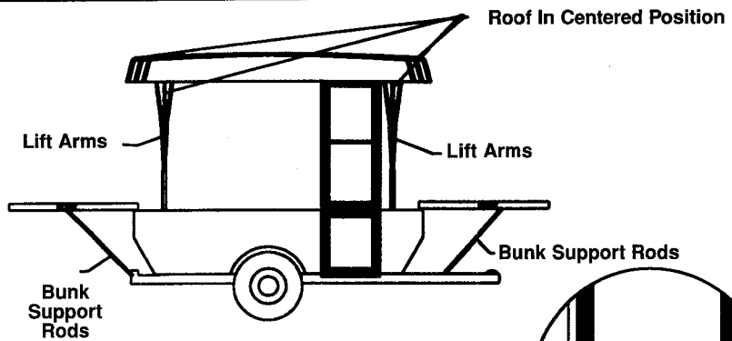
ROOF CENTERED POSITION
