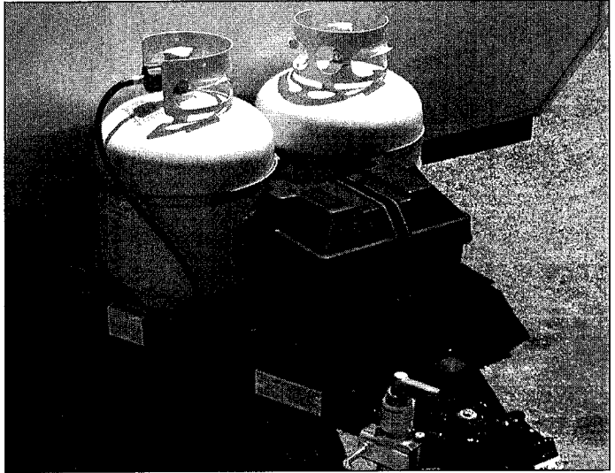
LPG HOSE ROUTING
